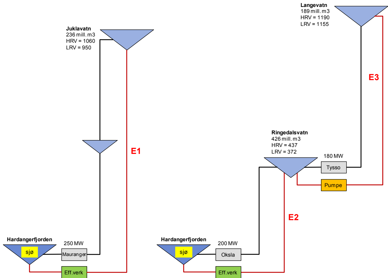
Figur 2.10: Case Mauranger (E1) – Oksla (E2) – Tysso (E3).
